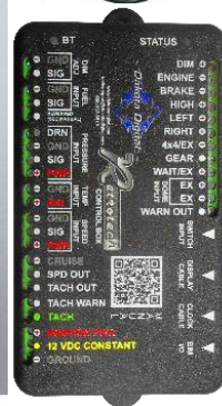
Control Box
