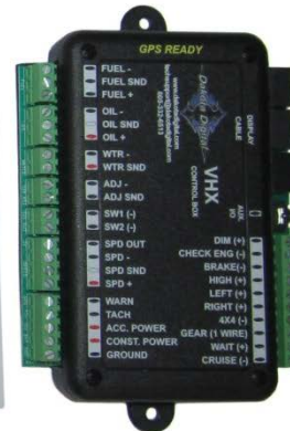
Control Box
